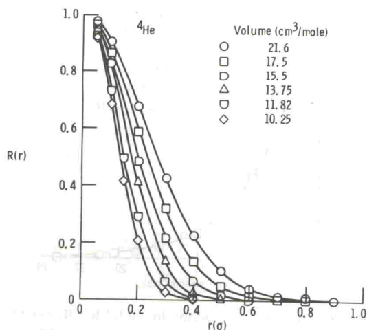
FIG. 10. Single-particle distribution function R(r) vs particle displacement from equilibrium for solid {}^4\text{He} at various volumes.
